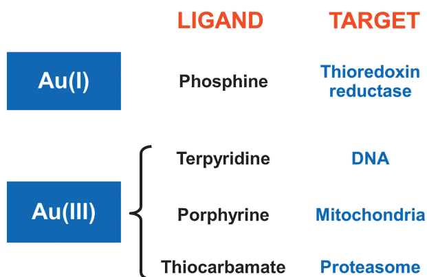
Fig. 16 – Overview of main ligand families used in Au(I) and Au(III) antitumor complexes and principal biological targets.
