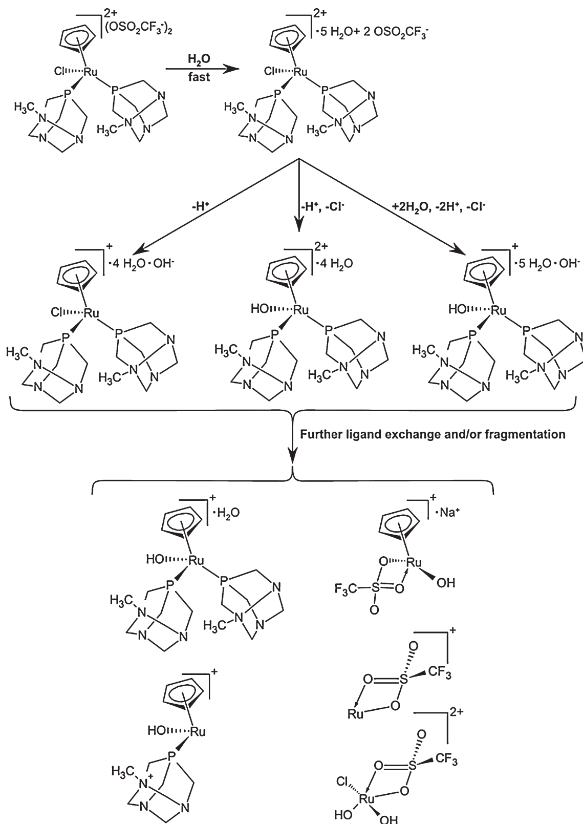
Fig. 13 – Scheme of [\text{RuCpCl}(\text{mPTA})_2](\text{OSO}_2\text{CF}_3)_2 hydrolysis as determined by mass spectrometric and spectrophotometric investigation.
