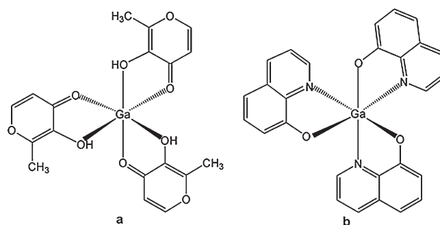
Fig. 20 – Structure of gallium maltolate (tris(3-hydroxy-2-methyl-4H-pyran-4-onato)gallium(III)) (a) and KP46 (tris(8-quinolonato)gallium(III)) (b).
