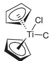
Fig. 21 – Structure of the titanocene dichloride.
