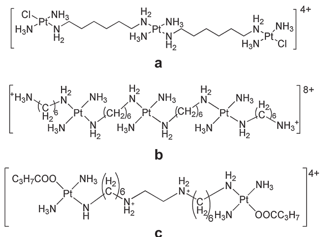
Fig. 7 – Structures of BBR3464 (a), [[\text{trans-Pt}(\text{NH}_3)_2(\text{NH}_2(\text{CH}_2)_6(\text{NH}_3^+))]]_2\text{-}\mu\text{-}[\text{trans-Pt}(\text{NH}_3)_2(\text{NH}_2(\text{CH}_2)_6\text{NH}_2)]_2^{8+} (b) and CT-47463 (c).
