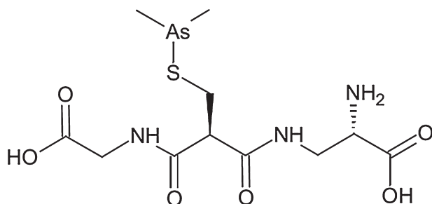
Fig. 22 – Structure of darinaparsin (S-dimethylarsino-glutathione).
