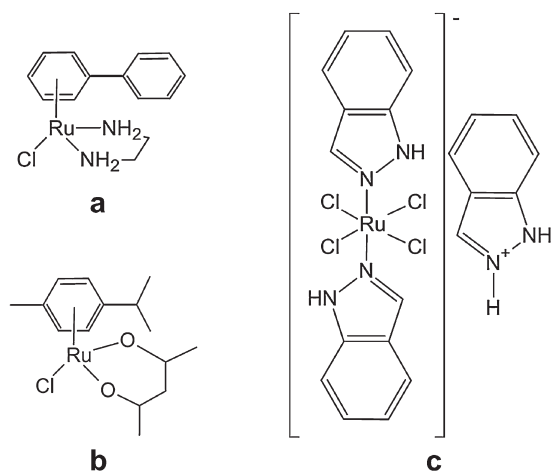
Fig. 11 – Structures of main Ru(II) and Ru(III) complexes: RM175 (a), [\text{Ru}(\eta^6\text{-p-cym})(\text{acac})\text{Cl}] ( p-cym = para -cymene) (b) and KP1019 (c).
