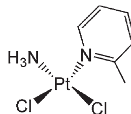
Fig. 4 – Structure of picoplatin (cis-amine-dichloro-(2-methylpyridine)-Pt(II)).
