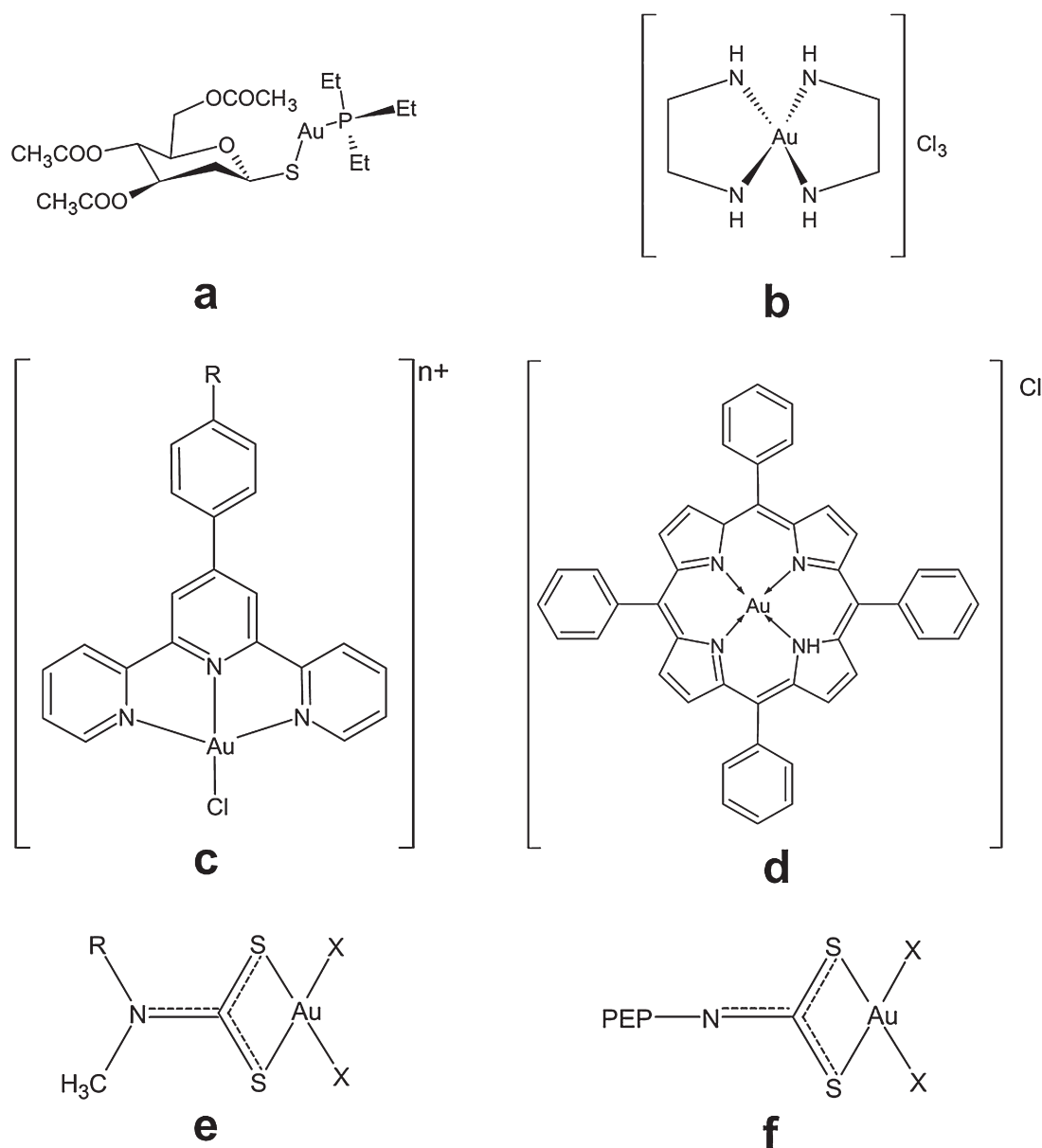
Fig. 15 – Structures of selected antitumor gold complexes: auranofin (a), [Au(en) 2 ] 2 Cl 3 (b), Au(III) complex with substituted terpyridine ligand (c), [Au(TPP)]Cl (H 2 TPP = tetraphenyl-porphyrin) (d), [Au(dtc)X 2 ] (X = Cl, Br; dtc = N,N-dimethyl-dithiocarbamate, ethyl-sarcosine-dithiocarbamate) (e) and [AuX 2 (pdtc)] (X = Cl, Br; pdtc = oligopeptide-dithiocarbamate, PEP-N is a di-, tri-, tetra- or penta-peptide) (f).
