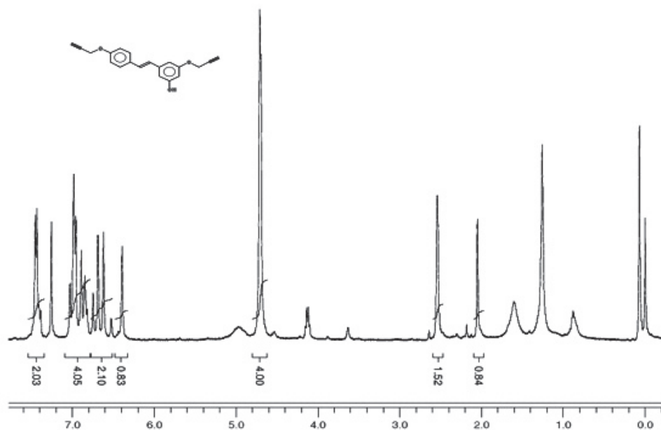
Supplementary Fig. 1. Assigned Spectra for RESL10 400 MHz 1 H Spectrum
